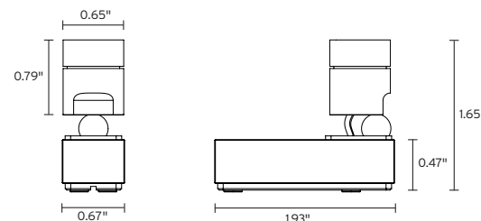
Fixture Dimensions
