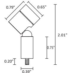
screw base
