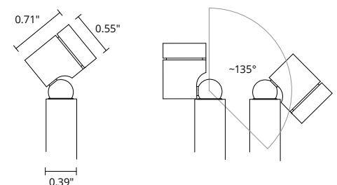
Fixture Dimensions
