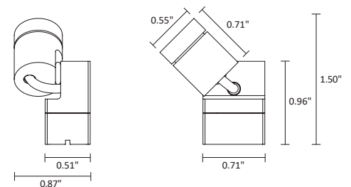
Fixture Dimensions
