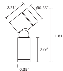
magnetic base
