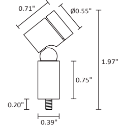
screw base
