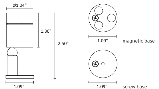
Fixture Dimensions
