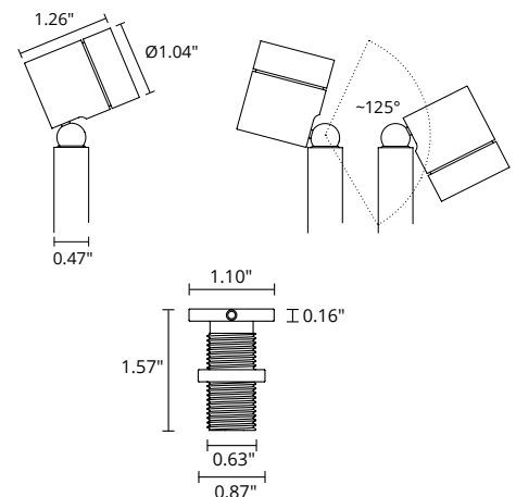
Fixture Dimensions
