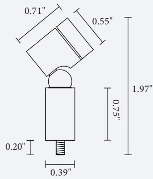
screw base (thread M3)
