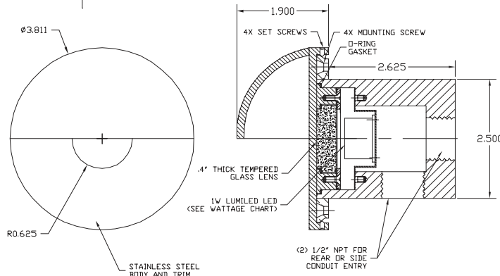
Fixture Dimensions
