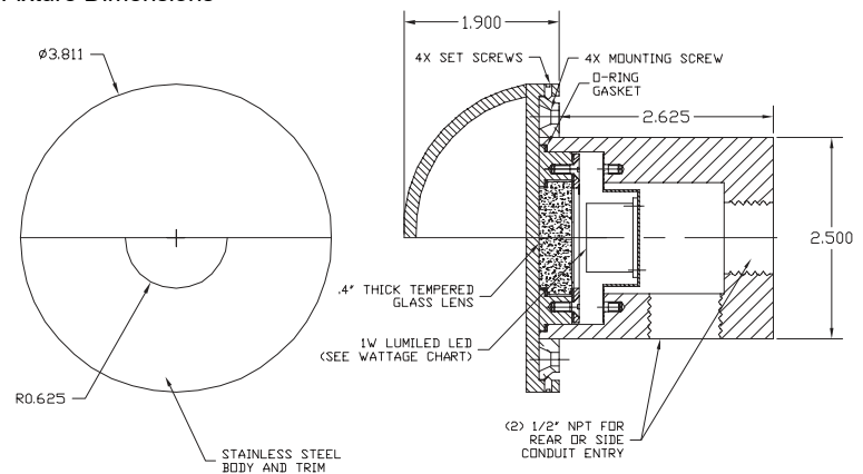
Fixture Dimensions
