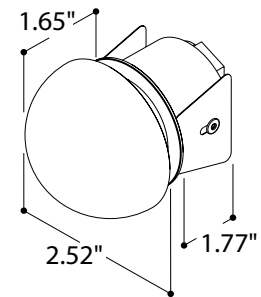
Fixture Dimensions
