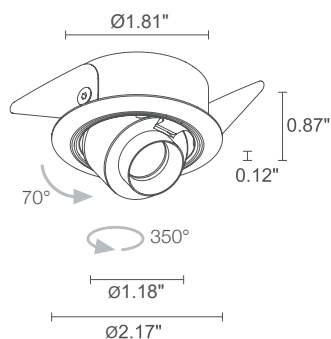
Ceiling Cut-Out: Ø1.97" Fixture Dimensions Ø1.18" x 0.87" h x Ø2.17" outer rim
