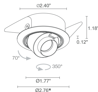
Ceiling Cut-Out: Ø2.56" Fixture Dimensions Ø2.40" x 1.18" h x Ø2.76" outer rim
