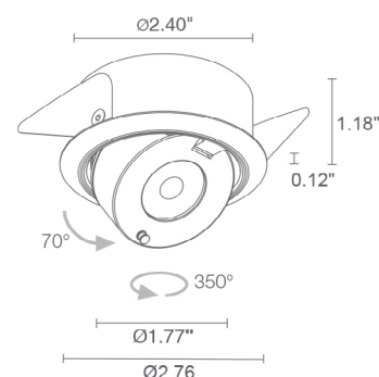
Ceiling Cut-Out: Ø2.56" Fixture Dimensions Ø2.40" x 1.18" h x Ø2.76" outer rim
