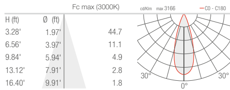
L - 33° CRI 90 - flat, round cover
