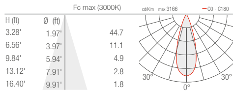
L - 33° CRI 90 - shallow, round cover
