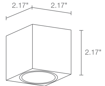
Fixture Dimensions
