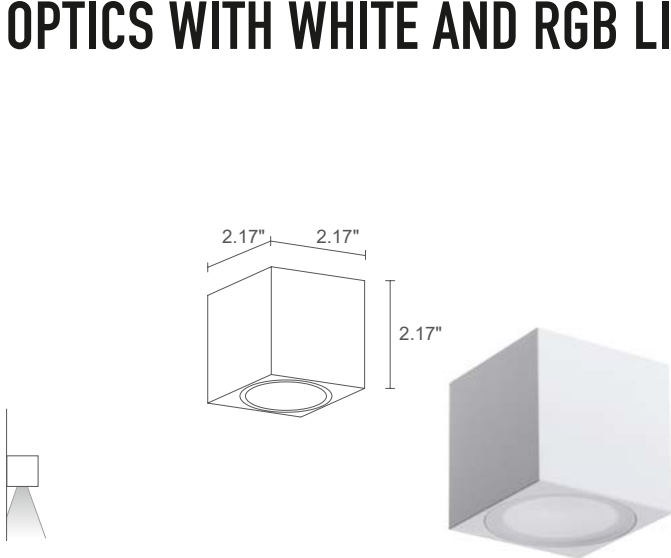
CUBE W 1.0
