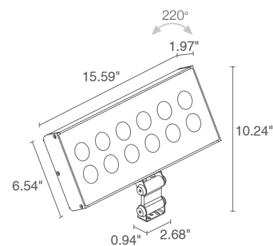
Fixture Dimensions
