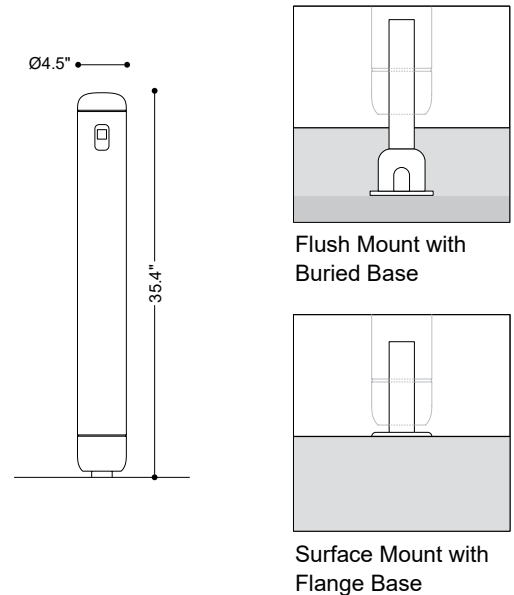
Fixture Dimensions Ø4.5" x 35.4" h
