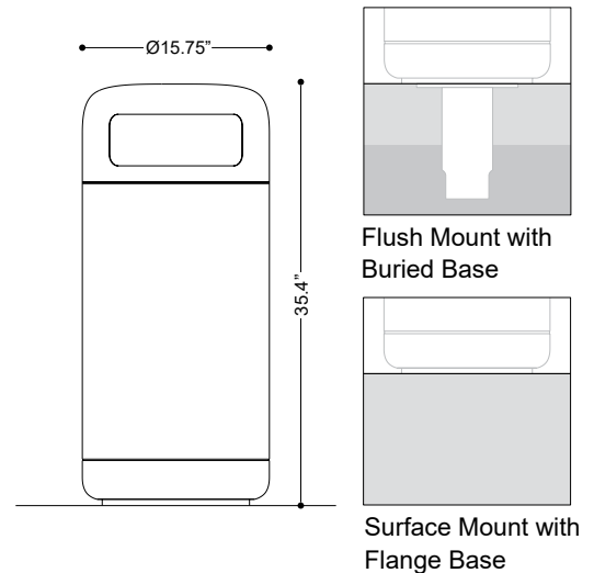
Fixture Dimensions Ø15.75" x 35.4"h
