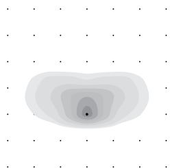
AS07 Asymmetric Side Throw
