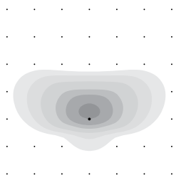
AS08 Asymmetric Side and Forward Throw
