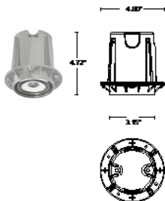
HOUSING BOX - Included
