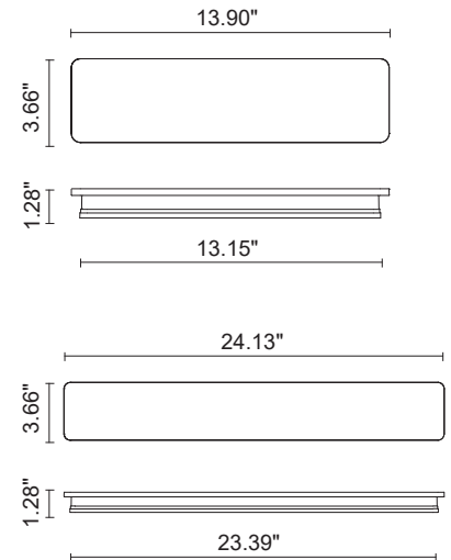
Fixture Dimensions
