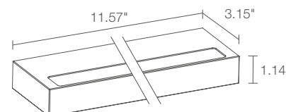
Fixture Dimensions
