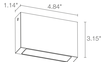
Fixture Dimensions
