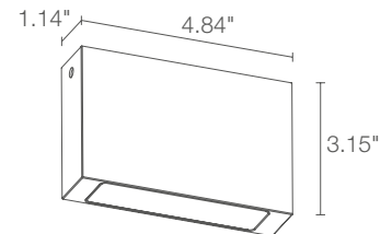
Fixture Dimensions
