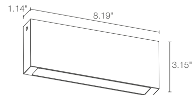
Fixture Dimensions
