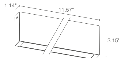
Fixture Dimensions
