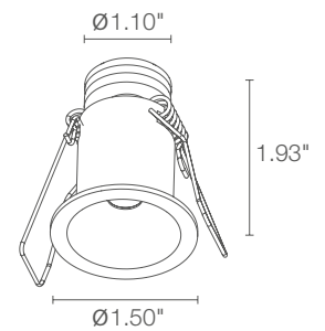
Ceiling Cut-Out: Ø1.18" Fixture Dimensions
