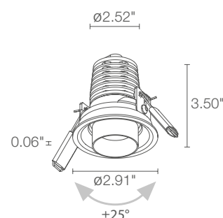
Ceiling Cut-Out: Ø2.56" Fixture Dimensions
