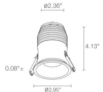
Ceiling Cut-Out: Ø2.56" Fixture Dimensions
