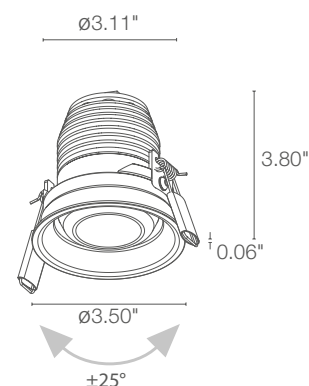
Ceiling Cut-Out: Ø3.15" Fixture Dimensions
