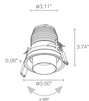
Ceiling Cut-Out: Ø3.15" Fixture Dimensions
