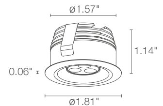
Ceiling Cut-Out: Ø1.61" Fixture Dimensions
