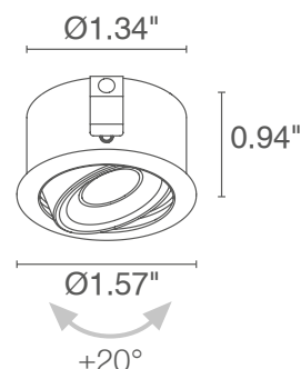
Ceiling Cut-Out: Ø1.38" Fixture Dimensions
