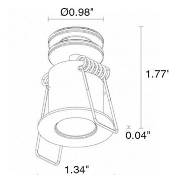
Ceiling Cut-Out: Ø1.18" Fixture Dimensions
