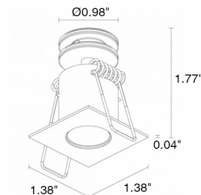
Ceiling Cut-Out: Ø1.18" Fixture Dimensions
