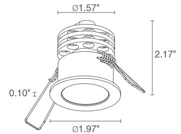
Ceiling Cut-Out: Ø 1.69" Fixture Dimensions
