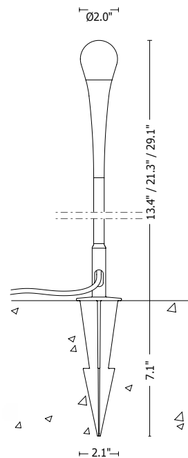
Mounting by spike
