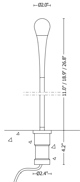
Mounting by housing box
