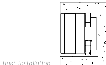
flush installation
