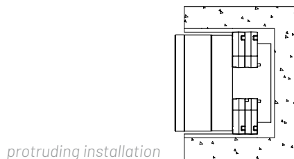
protruding installation
