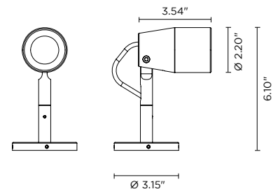
Fixture Dimensions:
