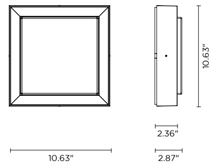
Fixture Dimensions:
