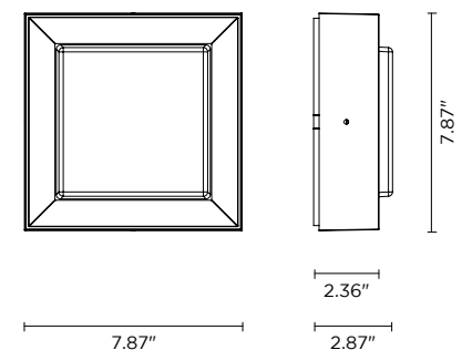
Fixture Dimensions:
