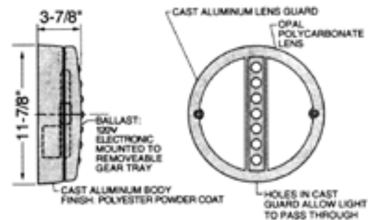
Fixture Dimensions
