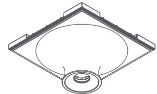
Ceiling Cut-Out: 15.9 x 15.9" Fixture Dimensions
