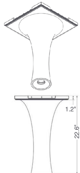
Ceiling Cut-Out: 15.9 x 15.9" Fixture Dimensions
