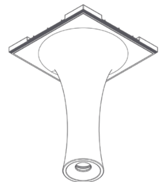
Ceiling Cut-Out: 15.9 x 15.9" Fixture Dimensions
