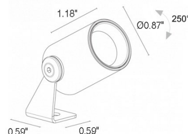
Fixture Dimensions
