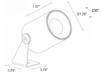
Fixture Dimensions
