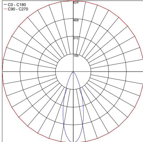
PHOTOMETRIC FILENAME : GEM 2.1 F 33° [3000K 4.5W 350MA].IES
