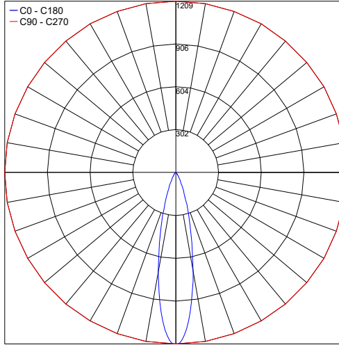
PHOTOMETRIC FILENAME : GEM 2.1 M 23° [3000K 4.5W 350MA].IES
