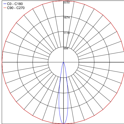
PHOTOMETRIC FILENAME : GEM 2.1 S 16° [3000K 4.5W 350MA].IES
