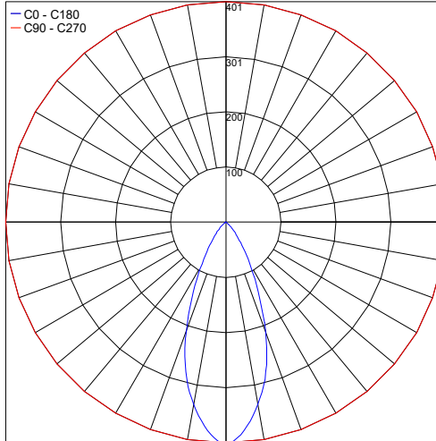
PHOTOMETRIC FILENAME : GEM 2.1 L 42° [3000K 4.5W 350MA].IES
