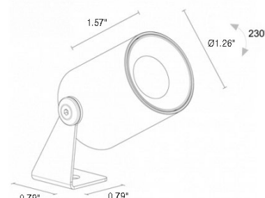
Fixture Dimensions
